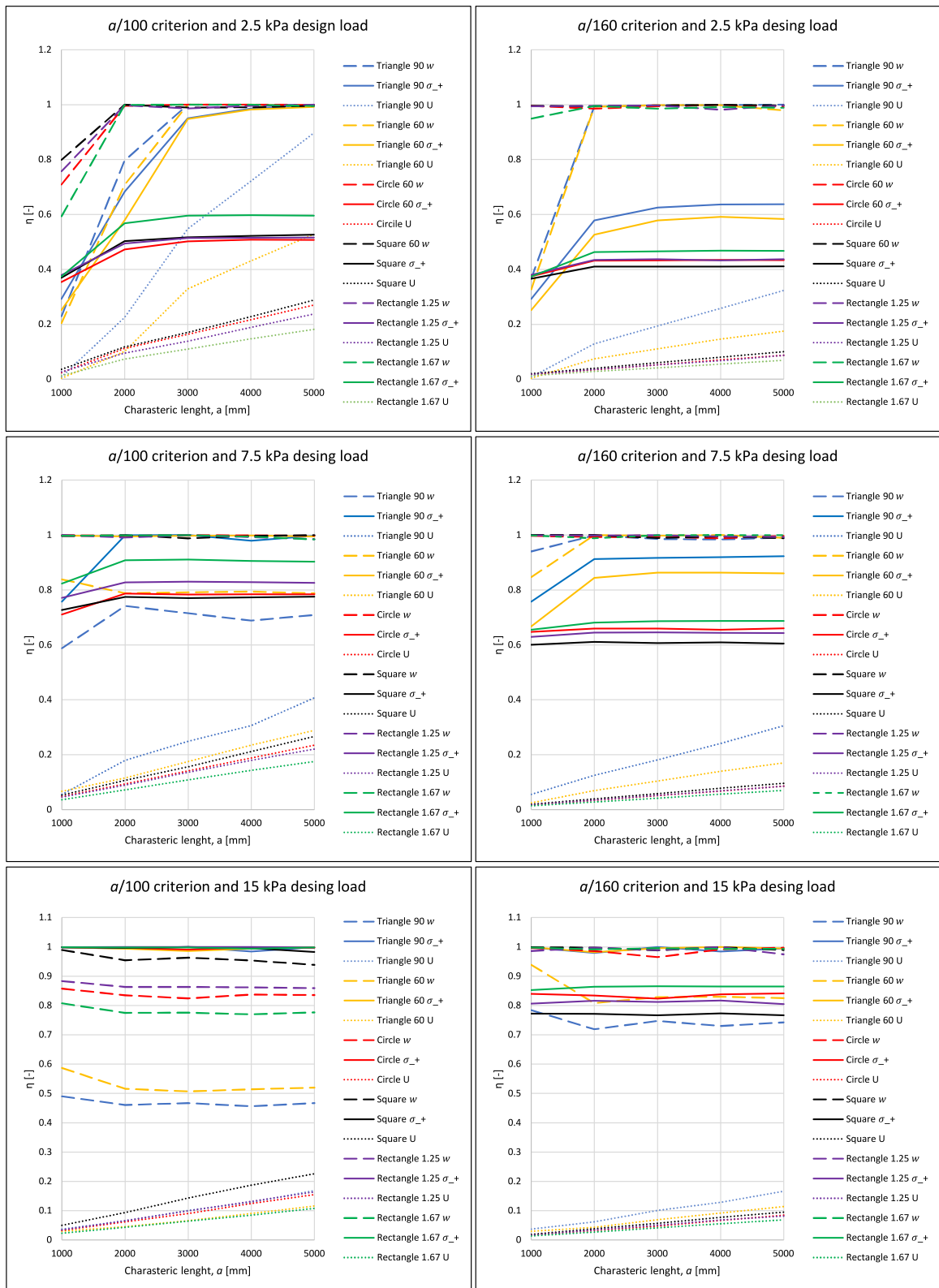
Fig. B.23. Activation of the design criteria in the exposed pane. The activation is \eta = response/criterion . Value of 1 means that the criterion has been reached. U is the maximum in-plane translation of the edge and w is maximum the deflection as shown in Fig. 3, and \sigma_+ is the maximum principal stress.
