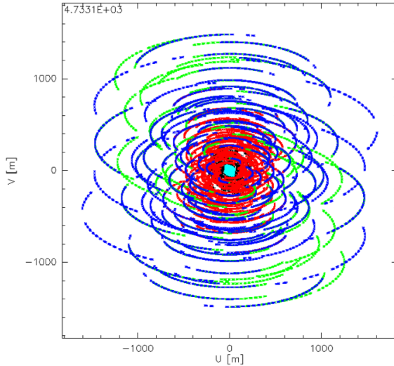
Figure 5.8: Combination of visibilities from different baseline configurations, shown in the uv plane. The red points indicate compact baselines, while the green and blue points show successively extended array configurations (credit: NRAO).
