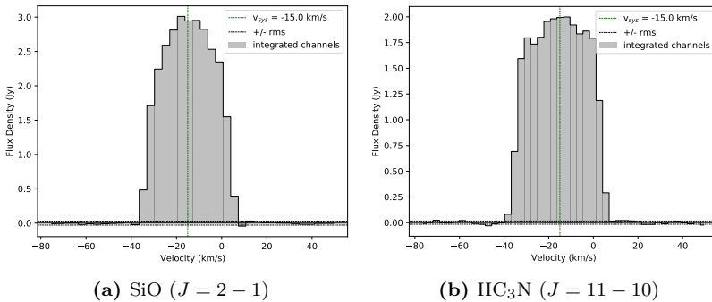
Figure 3.2: Spectral lines of the SiO ( J = 2 - 1 , left) and HC 3 N ( J = 11 - 10 , right) rotational transitions observed towards IRAS 15194–5115, using ALMA (credit: Unnikrishnan et al. 2023).
