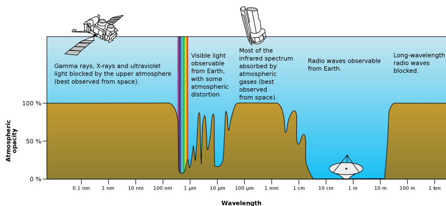
Figure 5.1: Opacity of the Earth’s atmosphere across the electromagnetic spectrum (credit: NASA).
