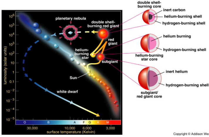
Figure 1.2: The evolutionary track of a 1 M_{\odot} star in the HR diagram, showing the stellar structure at various phases (credit: Pearson Education).
