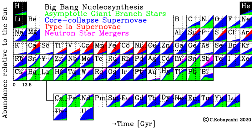
Figure 2.7: The periodic table of elements. Colours indicate different nucleosynthesis sources (credit: Kobayashi et al. 2020).
