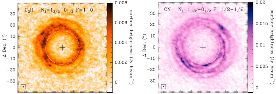
Figure 4.5: Systemic-velocity surface brightness maps of \text{C}_2\text{H} and \text{CN} towards IRC +10216, observed using ALMA (credit: Agúndez et al. 2017 ).
