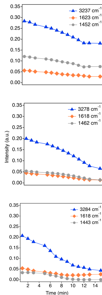
Figure 4.8: In situ DRIFT spectra peak intensity for pre-adsorbed NH 3 on different acid sites of the Cu-SSZ-13 (top), Cu-ZSM-5 (middle), and Cu-BEA (bottom) zeolites exposed to NO + NO 2 + O 2 at 200 °C.
