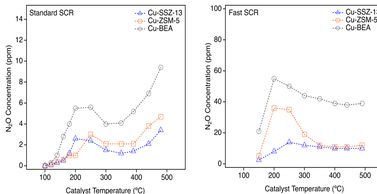
Figure 4.1: \text{N}_2\text{O} concentration as a function of catalyst temperature within standard and Fast SCR condition over Cu-based zeolites.
