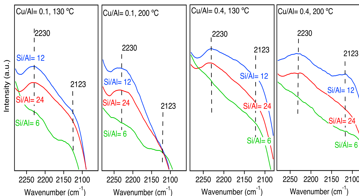
Figure 4.20: DRIFT spectra for the 5th min of the standard SCR over the sample with \text{Si/Al}= 12 and \text{Cu/Al}= 0.1 , and 0.4 molar ratio at 130\text{ }^\circ\text{C} .
