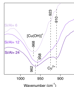
Figure 4.14: DRIFTS spectra of T-O-T vibrational region perturbed by \text{NH}_3 adsorption at 70 °C for Cu-SSZ-13 samples with Si/Al= 6, 12, and 24 and Cu/Al= 0.4 molar ratio.
