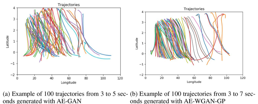
Fig. 10 The trajectories generated with AE-GAN and AE-WGAN-GP. (a): Trajectories of length 3 to 5 seconds, and (b): trajectories of length 3 to 7 seconds
