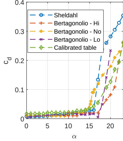
(b) 2D drag coefficient
