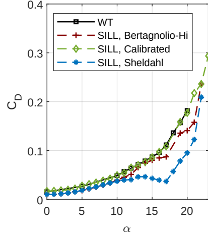
(b) 3D drag coefficient
