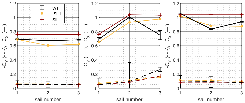
(a) Validation case T20 where the sails are equally sheeted to \alpha_1 = 10^\circ , \alpha_2 = 15^\circ and \alpha_3 = 15^\circ , generates the highest driving force. (b) Validation case T25 , where the sails are equally sheeted to \alpha_1 = \alpha_2 = \alpha_3 = 10^\circ . Sail 3 has stalled. (c) Validation case T28 , where the sails are equally sheeted to \alpha_1 = \alpha_2 = \alpha_3 = 15^\circ , generates the highest driving force.
