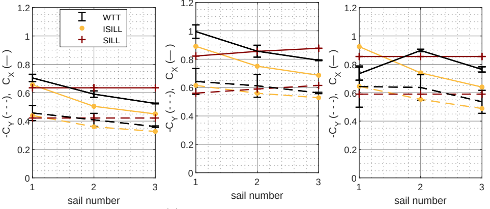
(a) Validation case T20 where the sails are equally sheeted to angles \alpha_1 = \alpha_2 = \alpha_3 = 10^\circ . (b) Validation case T27 , where \alpha_1 = 14^\circ , \alpha_2 = 15^\circ and \alpha_3 = 16^\circ generates the highest driving force. (c) Validation case T28 where \alpha_1 = \alpha_2 = \alpha_3 = 15^\circ . Sail 1 has stalled in the wind tunnel tests.
