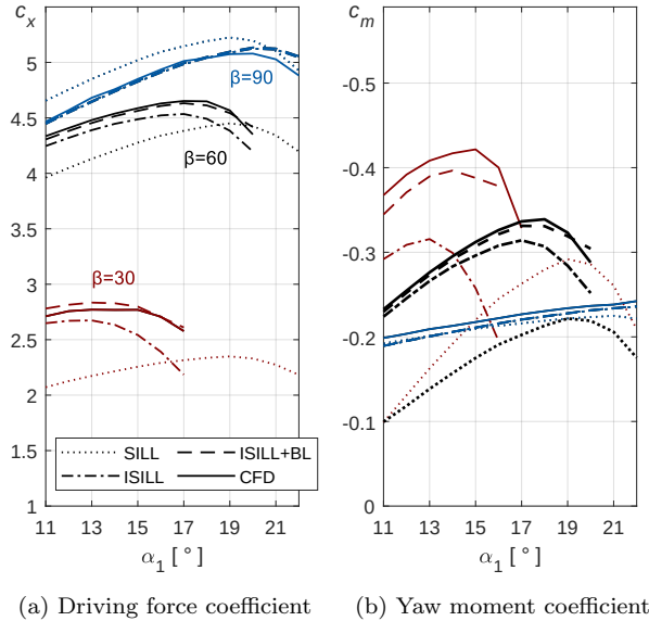
Figure 4.6: 2D sheeting sweep for \beta_{AW} = 30^\circ, 60^\circ and 90^\circ where Sail 1 (fore) is swept from a low to a high angle of attack. For sheeting angles of Sail 2 and Sail 3; see validation cases 2.1, 2.4 and 2.7 in Table 4.2.
