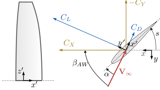
Figure 2.1: Definitions of the coordinate systems, force vectors, apparent wind angle \beta_{AW} , angle of attack \alpha and sheeting angle s . The apparent wind is indicated by the red arrow.
