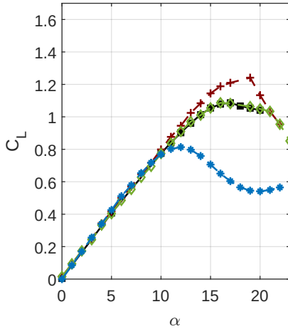
(a) 3D lift coefficient
