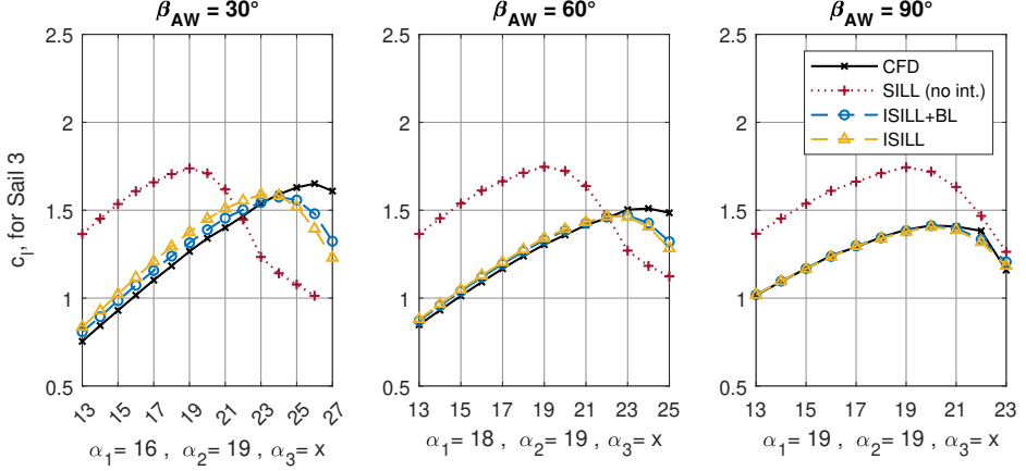
Figure 4.5: Lift coefficient for Sail 3 when sailing at \beta_{AW} = 30 (v.c. 2.3), \beta_{AW} = 60 (v.c. 2.6) and \beta_{AW} = 90 (v.c. 2.9). The aftmost profile (Sail 3) is swept from a low to a high angle of attack, whilst the other two profiles are kept stationary.
