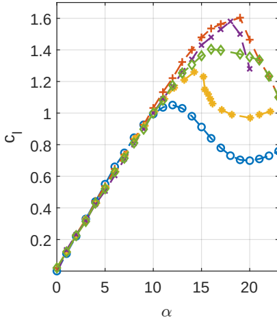
(a) 2D lift coefficient
