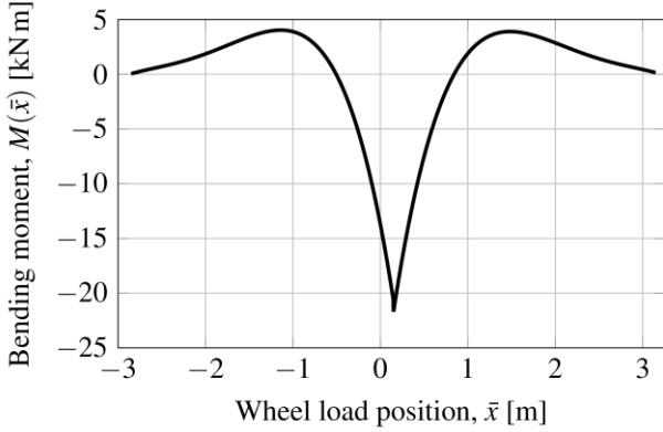
Figure 2 Evolution of bending moment at the position of crack mouth as a function of the relative position of the wheel. Results from the vehicle-track simulation software DIFF [15].
