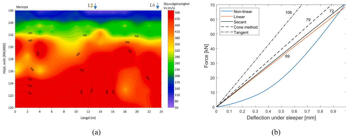
Fig. 2. Measured shear wave speed distribution of layered soil (from Ref. [44]), and (b) calculated force–displacement characteristic for foundation support stiffness at Gransjö. Linear(ised) stiffness values [kN/mm] per sleeper are indicated in the figure.
