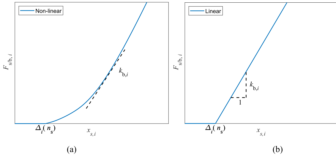
Fig. 6. Principle illustration of two alternative force–displacement characteristics for the spring modelling the foundation support stiffness (a) non-linear force–displacement, (b) piecewise linear force–displacement.
