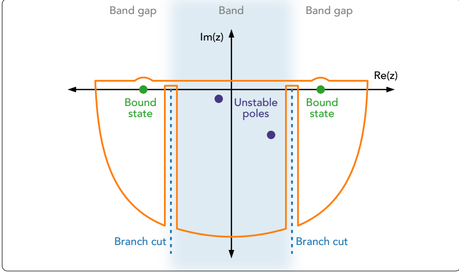
Figure 3.1: Contour of the integral in Eq. (3.43), with contributions from the poles of the resolvent [Eq. (3.42)] and the branch cuts at the band edges ( |\text{Re}(z)/J| = 2 ). Figure extracted from Paper B and inspired by Ref. [110].
