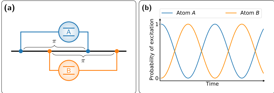
Figure 2.3: (a) Two braided giant atoms with the coupling points of each atom separated by a phase shift of \pi \pmod{2\pi} , which is the distance that allows them to interact without decohering. (b) Excitation exchange between two atoms arranged in the setup from (a), showing a decoherence-free interaction.
