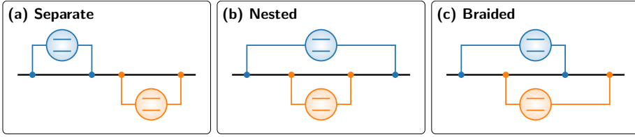
Figure 1.2: Different arrangements of two giant atoms with two coupling points each. Figure adapted from Paper B.
