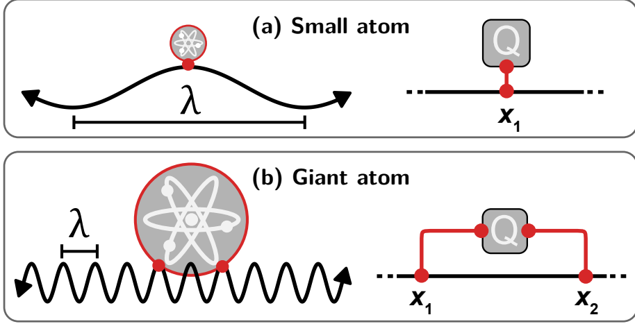
Figure 1.1: (a) A small atom, treated as a point-like object because it is much smaller than the wavelength \lambda of the field it interacts with. (b) A giant atom, formed by coupling a small atom to a mode at two discrete locations, spaced wavelengths apart. Figure adapted with permission from Ref. [12].
