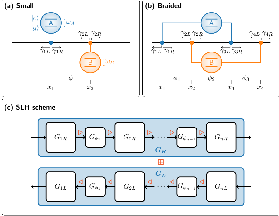
Figure 2.2: Atoms coupled to a 1D continuous open waveguide. (a, b) A sketch for (a) two small atoms, and (b) two giant braided atoms showing the relevant parameters. (c) The SLH scheme that describes the input-output flows from the setups in (a) and (b), and which is also applicable to an arbitrary number of atoms with an arbitrary number of coupling points. All figures are adapted from Paper A.
