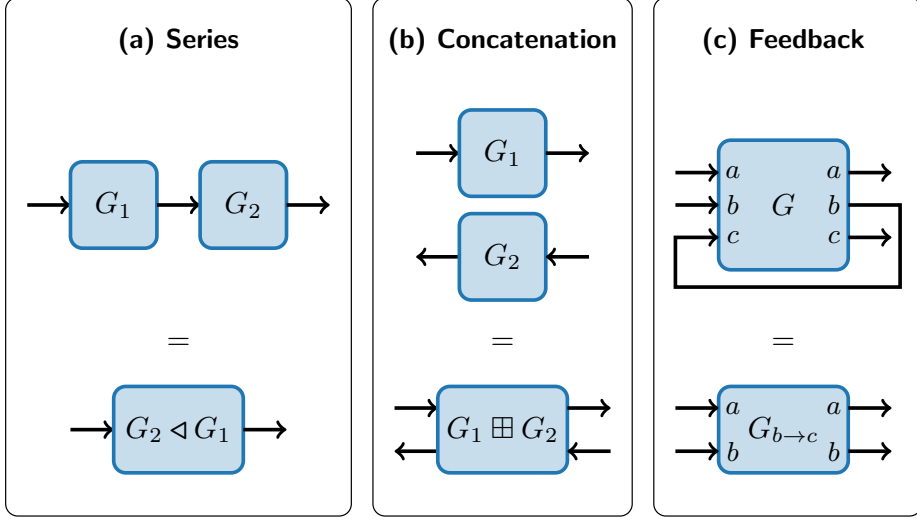
Figure 2.1: The three SLH composition rules: (a) series product, (b) concatenation product, (c) feedback operation.
