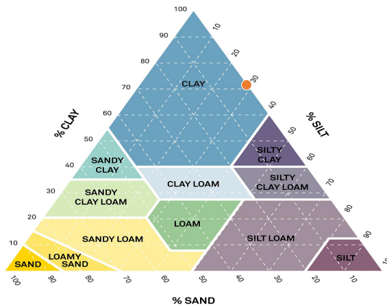
Figure 4.1: Composition of Kärä clay from 9 m depth.
