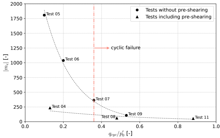
Figure 5.5: Relationship between the degree of shear mobilisation ( q_{cyc}/p'_0 ) and the resistance number ( m_e ) for Kärä samples obtained from undrained cyclic triaxial tests.
