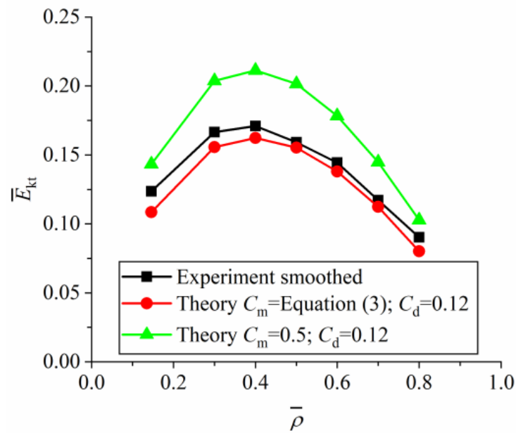
Figure 14. Dimensionless kinetic energy \bar{E}_{kt} of the sphere just before contacting the ice plate versus the relative density obtained by three methods with \bar{h} = 0.089 and \bar{L}_0 = 2.31 constant.
