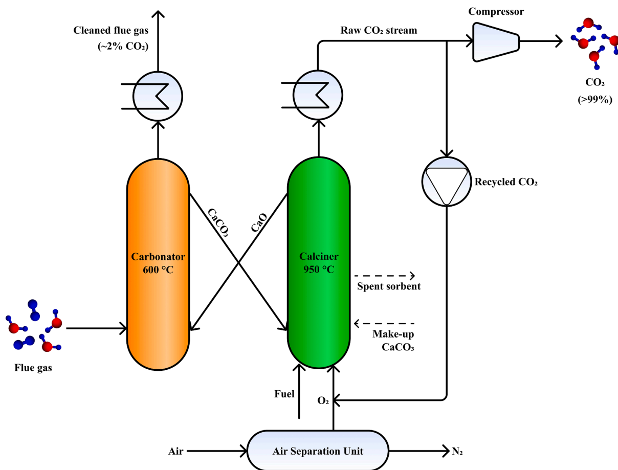
Fig. 19. CO 2 capture from flue gas by calcium looping process (CaL).
