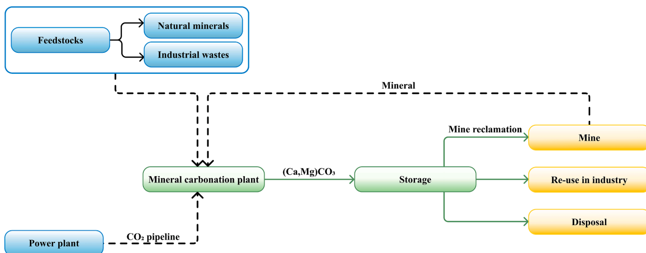
Fig. 29. Illustration of CCMC technology steps.
