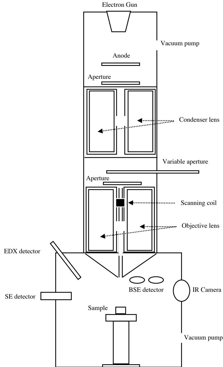
Figure 6.1: Schematic representation of a SEM.
