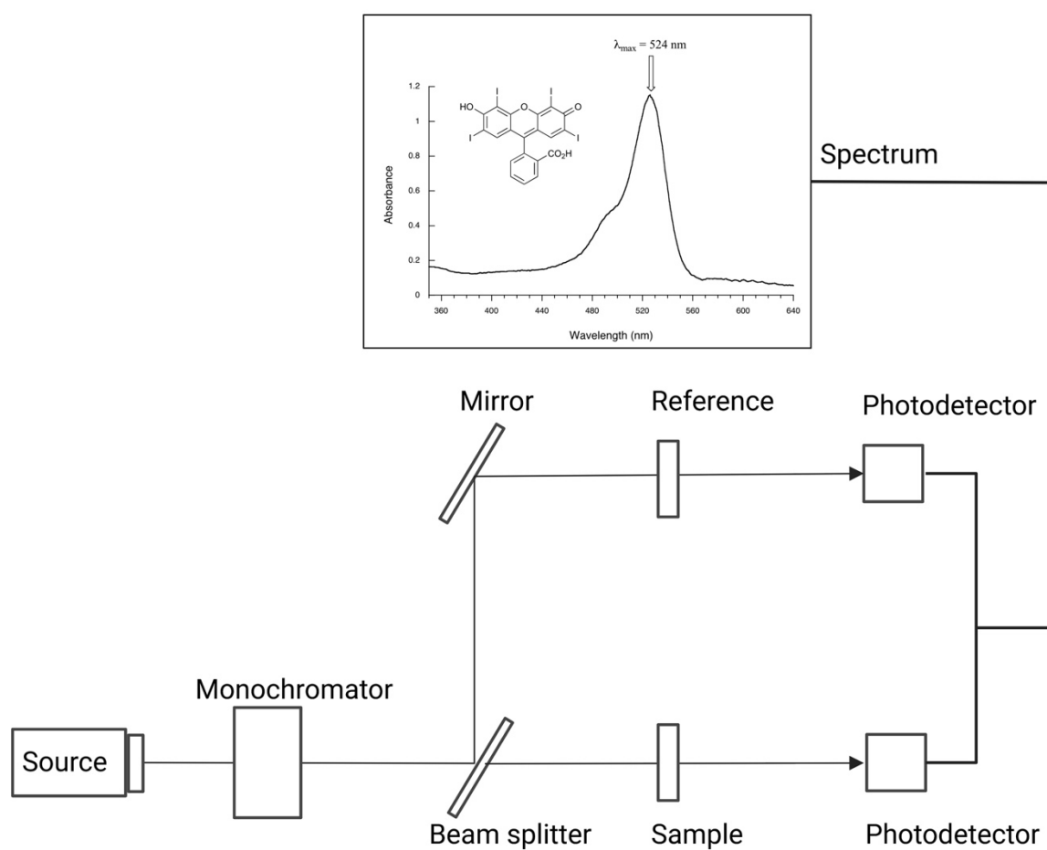
Figure 6.7: Schematic representation of an UV-Vis instrument with a double beam setup. It also provides an example of an spectra of a molecule.
