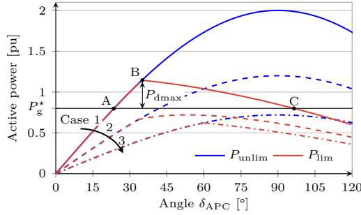
Figure 3.3: P - \delta_{APC} curve illustrating the converter angle stability problem for a current limit of 1.2 pu. A: pre-disturbance operating point; B: current limit reached; C: transient stability limit; P_{dmax} : maximum decelerating power; all outlined for case 1: E_{EMF} = E_s = 1.0 pu. Case 2: E_{EMF} = 1.0 pu & E_s = 0.6 pu; case 3: E_{EMF} = E_s = 0.6 pu.
