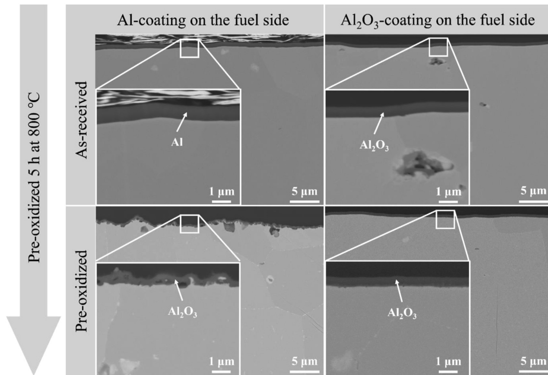
Fig. 7 – Effect of the pre-oxidation step on metallic Al coating. Top panel: As-received Al-coated and \text{Al}_2\text{O}_3 -coated 441 steel. Bottom panel: The same surface after 5 h of pre-oxidation with up and down ramp rates of 1^\circ\text{C}/\text{min} in humid (3% water vapour) laboratory air at 800^\circ\text{C} .
