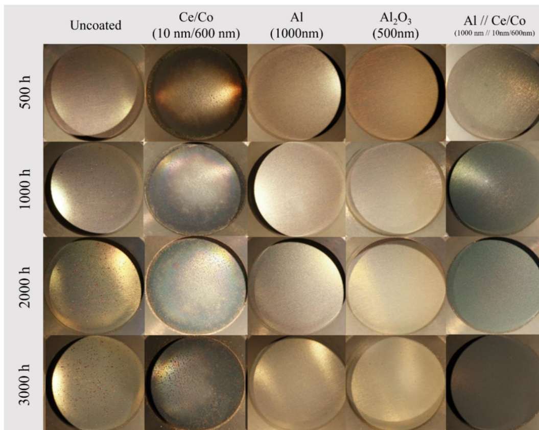
Fig. 1 – Photographs of the air-facing sides of AISI 441 coupons taken during exposure to a discontinuous dual-atmosphere ( \text{Ar}-5\% \text{ H}_2 + 3\% \text{ H}_2\text{O} // \text{Air} + 3\% \text{ H}_2\text{O} ) at 600 \text{ }^\circ\text{C} .
