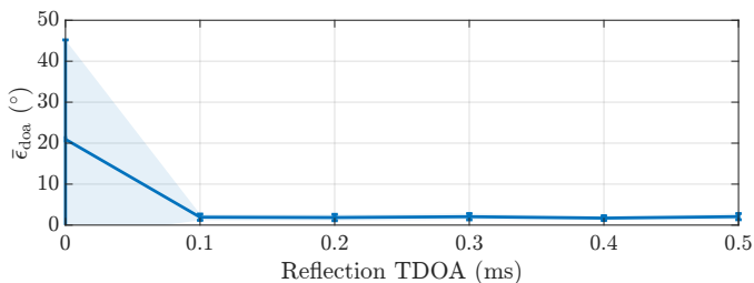
Fig. 9. Means and standard deviations of the average DOA estimation error \bar{\epsilon}_{\text{doa}} for two simultaneously arriving reflections, Array2 and different TDOAs.
