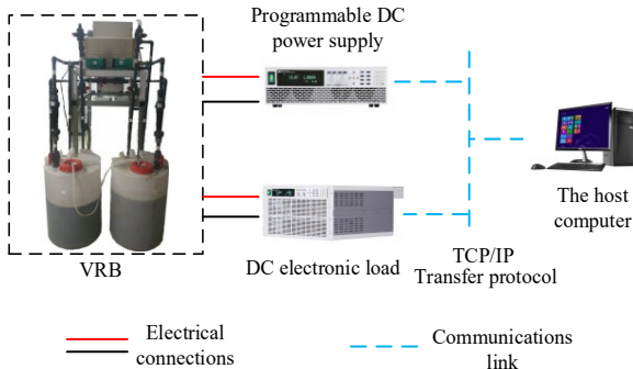
Fig. 3. Schematic of the VRB experimental setup.
