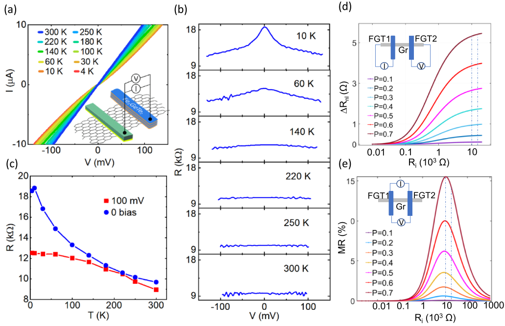
Figure 3. Electrical characterization and magnetoresistance calculation for the graphene/FGT van der Waals heterostructure. (a) Current–voltage characteristic of the graphene/FGT heterostructure with measurement geometry shown in the inset. (b) Differential resistance of graphene/FGT structure as a function of bias at different temperatures. (c) Temperature dependence of resistance at zero and 100 mV bias voltages. (d), (e) Calculated nonlocal and local spin valve signal magnitude as a function of the interface resistance ( R_i ) with different effective spin polarization of FGT. The x-axis is in a log scale.
