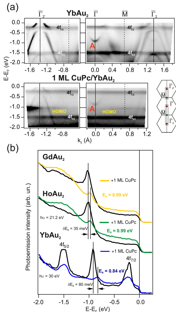
Fig. 4 Representative ARPES band structure of \text{REAu}_2 surfaces compounds before and after CuPc adsorption. (a) Photoemission intensity mapping taken along the indicated \bar{\Gamma}\bar{M} directions of \text{YbAu}_2 (top) and 1 ML CuPc on \text{YbAu}_2 . The non-dispersing HOMO levels of CuPc add to the substrate bands after adsorption ( h\nu = 30 \text{ eV} ). (b) Upshift of the A band upon adsorption of 1 ML of CuPc on \text{YbAu}_2 , \text{HoAu}_2 and \text{GdAu}_2 . The largest shift has been detected in the \text{YbAu}_2 surface compound ( \theta = 0 , h\nu = 30 \text{ eV} [ \text{YbAu}_2 ], 21.2 \text{ eV} [other]).
