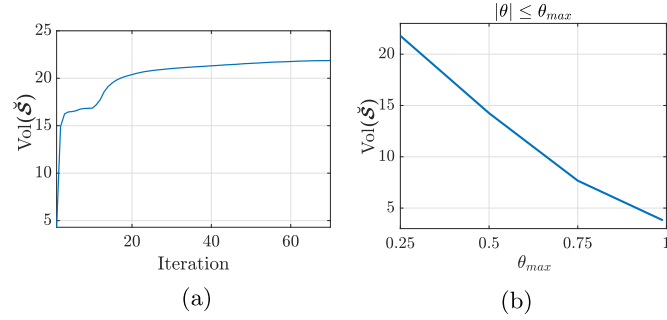
Fig. 3. Volume of the set \check{\mathcal{S}} plotted against (a) iteration, (b) different scheduling parameter bounds.
