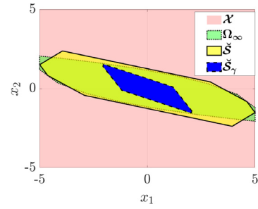
Fig. 4. Admissible set \mathcal{X} (red), maximal RCI set \Omega_\infty (green), and RCI sets \check{\mathcal{S}} (yellow) and \check{\mathcal{S}}_\gamma (blue). (For interpretation of the references to color in this figure legend, the reader is referred to the web version of this article.)
