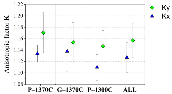
Figure 7. Data calculated from calliper dimensional measurements of the BJT samples studied: (a) sintered averaged shrinkages of the sintered samples along each direction and (b) averaged anisotropic factors calculated from the sintered shrinkage measurements. (SV samples results).
