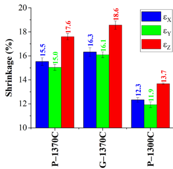
Figure 7. Data calculated from calliper dimensional measurements of the BJT samples studied: (a) sintered averaged shrinkages of the sintered samples along each direction and (b) averaged anisotropic factors calculated from the sintered shrinkage measurements. (SV samples results).
