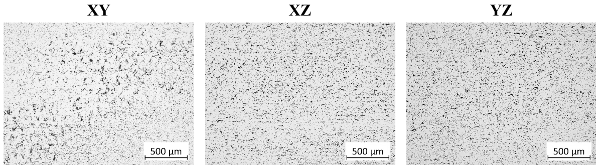
Figure 9. XY, XZ and YZ cross-section LOM images from samples sintered up to 1300°C. (SV samples results).
