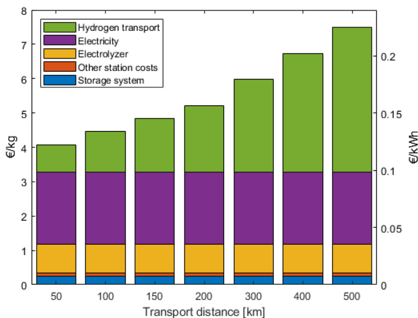
Fig. 9 – Costs for hydrogen from the Centralized, grid-connected system (Cen-Gc) and the current timeframe applying different average hydrogen transport distances from the production site to the refueling station.
