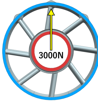
Figure 3.4: Depiction of load case used to test structural performance of a turbine rear structure under fan-blade-out conditions.
