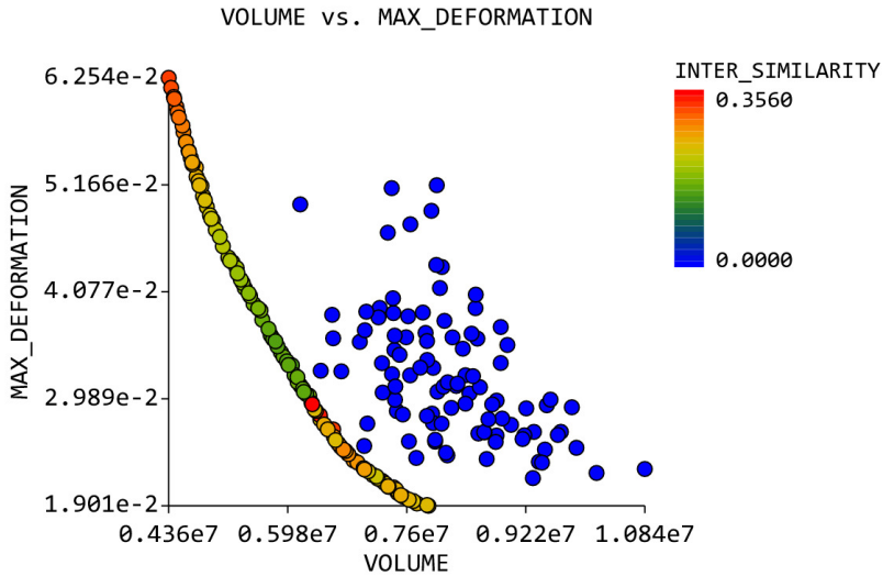
Figure 4.7: Results from an optimization study where inter-similarity is used to indicate the trustworthiness of the surrogate model results (the trade-off curve) through color-coding.
