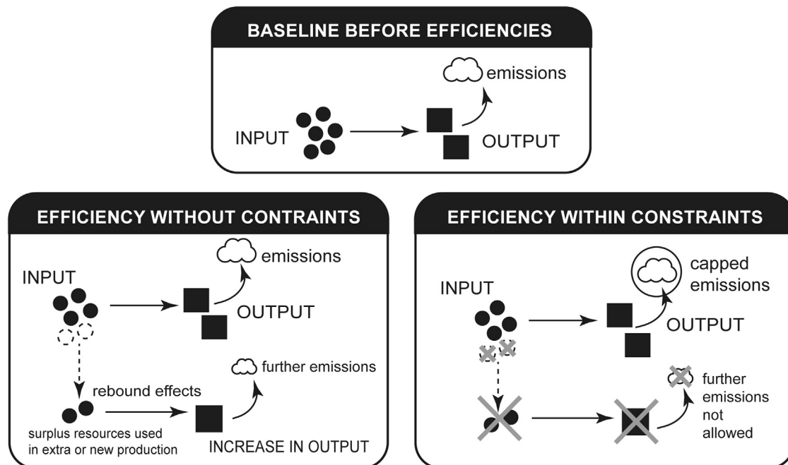
Figure 2. A visualization of rebound effects from efficiency and efficiency under emissions constraints
