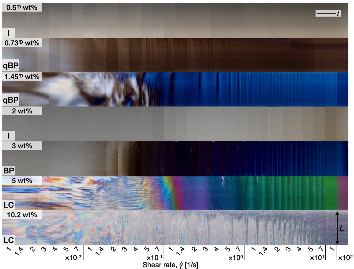
Fig. 5. Space-time optical visualization from the steady shear tests for all investigated CNC concentrations showing the birefringence patterns.
