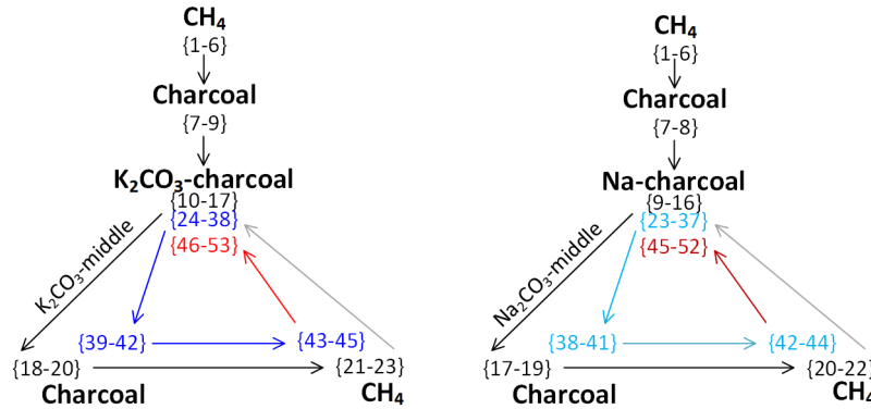
Figure 2. The two series of experiments with e.g. (a) K_2CO_3 -charcoal and (b) Na_2CO_3 -charcoal. The consecutive cycle numbers are presented in brackets. Arrows show the experimental flow stream.
