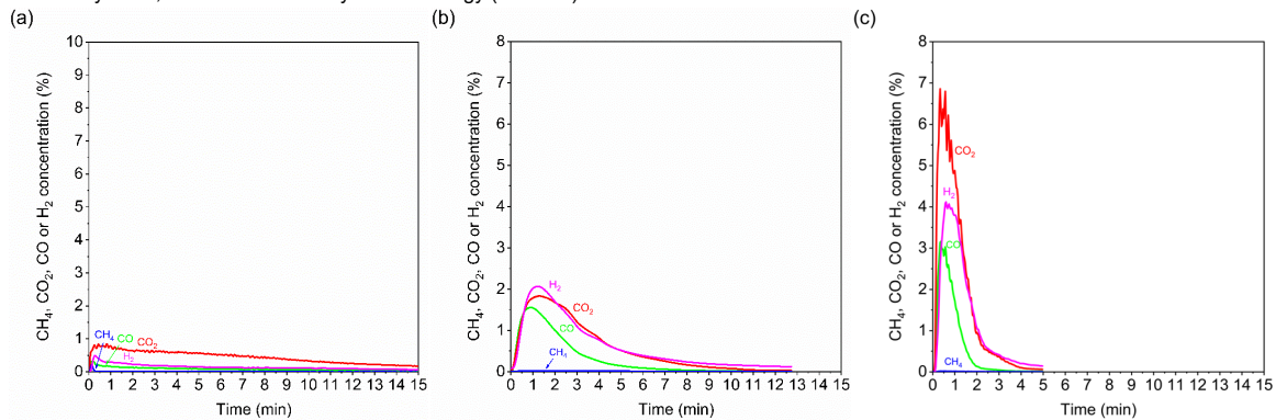
Figure 4. Concentrations of \text{CH}_4 , \text{CO} , \text{CO}_2 and \text{H}_2 during the braunite reduction with (a) charcoal, (b) KCl-charcoal and (c) \text{K}_2\text{CO}_3 -charcoal at 950^\circ\text{C} under the fluidization with 48% \text{H}_2\text{O} +52% \text{N}_2 .
