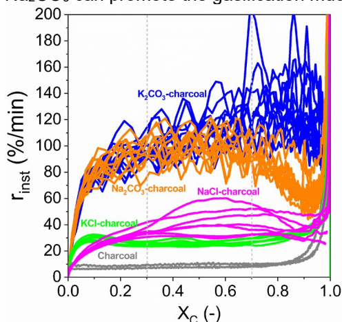
Figure 5. Rate of char gasification as a function of carbon conversion for charcoal, KCl-charcoal, NaCl-charcoal, \text{K}_2\text{CO}_3 -charcoal and \text{Na}_2\text{CO}_3 -charcoal. Different curves in a same colour show the cycle number with a specific fuel.
