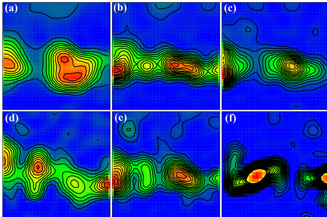
Fig. 14. \varphi_2 = 45^\circ ODF maps of the un-recrystallized fraction for specimens with different recrystallized fractions, (a) X_{REX}=13.5\% , (b) X_{REX}=57.6\% , (c) X_{REX}=76.1\% , (d) X_{REX}=80.3\% , (e) X_{REX}=89.1\% , (f) X_{REX}=95.7\% . Contour levels: 1 \times .
