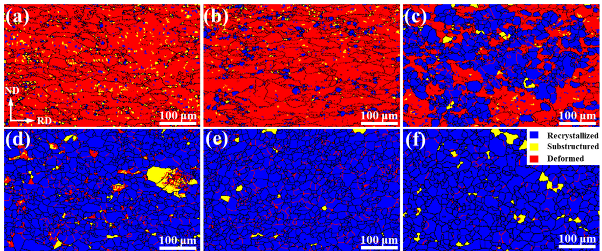
Fig. 4. Determining the recrystallization temperature of cold pilgered FeCrAl cladding tube, based on the EBSD recrystallization fraction map including (a) 700 °C, (b) 730 °C, (c) 760 °C, (d) 800 °C, (e) 850 °C and (f) 900 °C. The annealing time is 30 min for all the samples.
