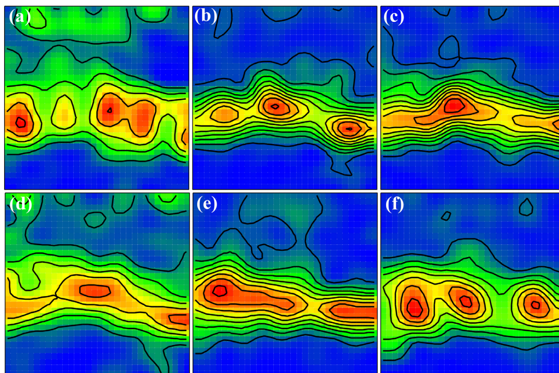
Fig. 15. \varphi_2 = 45^\circ ODF section maps of the recrystallized fraction specimens with different recrystallized Please check funding information and confirm its correctness.fractions, (a) X_{REX}=13.5\% , (b) X_{REX}=57.6\% , (c) X_{REX}=76.1\% , (d) X_{REX}=80.3\% , (e) X_{REX}=89.1\% , (f) X_{REX}=95.7\% . Contour levels: 1^\circ .
