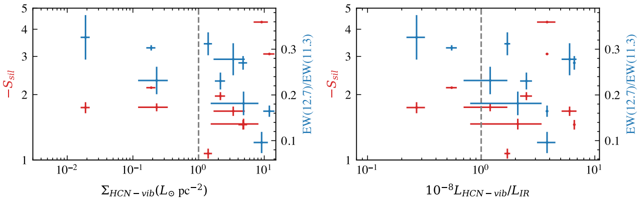
Fig. C.1. Same as Fig. 7 but with the apparent silicate strength as calculated by Eq. 6 (red), which shows no trend. The 12.7/11.3 PAH EW ratio is also shown (blue) against HCN-vib on the right-hand axis of each plot and shows a very weak trend. A comparison with Fig. 7 shows the value in accounting for the star-forming contribution to properly recover properties of the obscured nucleus.
