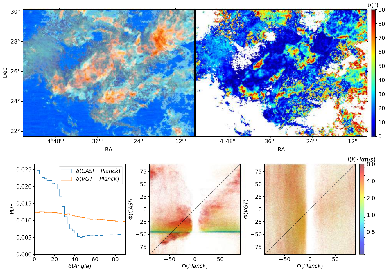
Figure 10. Upper left: integrated ^{12}\text{CO} emission overlaid with gray shadows indicating the location where CASI-3D predicted magnetic field directions are similar to those inferred by Planck dust polarized emission. Upper right: angle difference between the CASI-3D predicted magnetic field directions and those inferred by Planck dust polarized emission. Lower left: distribution of the angle difference between the CASI-3D predicted magnetic field directions and those inferred by Planck, and the angle difference between velocity channel gradient (VGT) inferred magnetic field directions and those inferred by Planck. Lower middle: scatter plot between the Planck dust polarization inferred magnetic field directions \Phi_{\text{Planck}} and the CASI-3D predicted directions \Phi_{\text{CASI}} . Lower right: scatter plot between the Planck dust polarization inferred magnetic field directions \Phi_{\text{Planck}} and the VGT predicted directions \Phi_{\text{VGT}} . The color in the scatter plots indicate the integrated intensity of ^{12}\text{CO} at each pixel.
