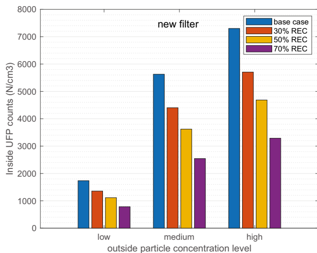
Fig. 13 Steady state inside UFP counts at three outside concentration levels, grouped with different recirculation degrees, in comparison with base case. Low, medium, and high stand for outside PM_{2.5} con-
