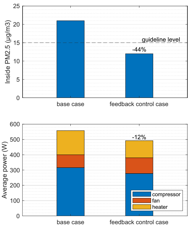
Fig. 11 Comparison of base case and feedback control case results of steady state PM 2.5 concentration and case-averaged power. Ambient condition T27, medium outside particle concentration level, aged filter, and 1 passenger
