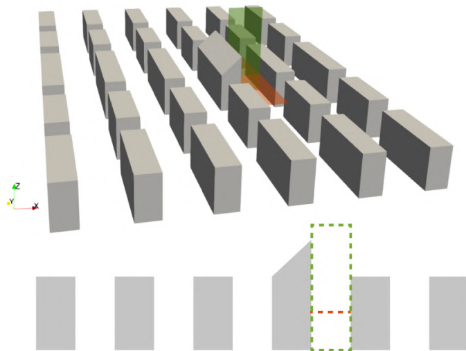
Figure 4.1: Top: 3D visualization of the domain where the red and green planes show the horizontal and vertical PIV-planes, respectively. Bottom: 2D side view, PIV-planes showed as dashed lines in green and red.
