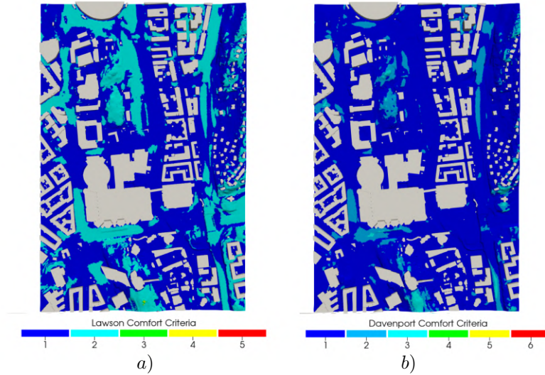
Figure 4.5: a) Lawson comfort criteria based on hourly data over one year. b) Davenport comfort criteria based on hourly data over one year. Both shown at pedestrian height.
