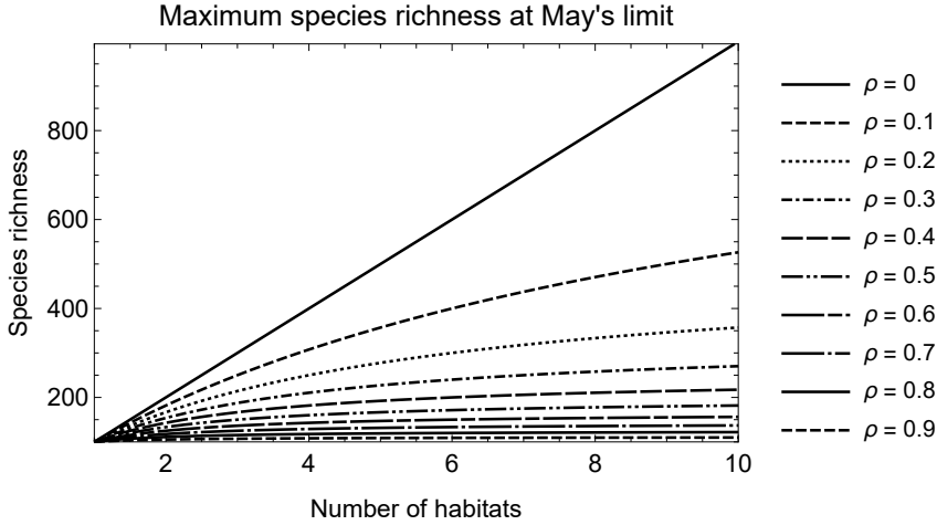
Figure 3.7: Maximum species richness increases with number of habitats and decreasing correlation.
