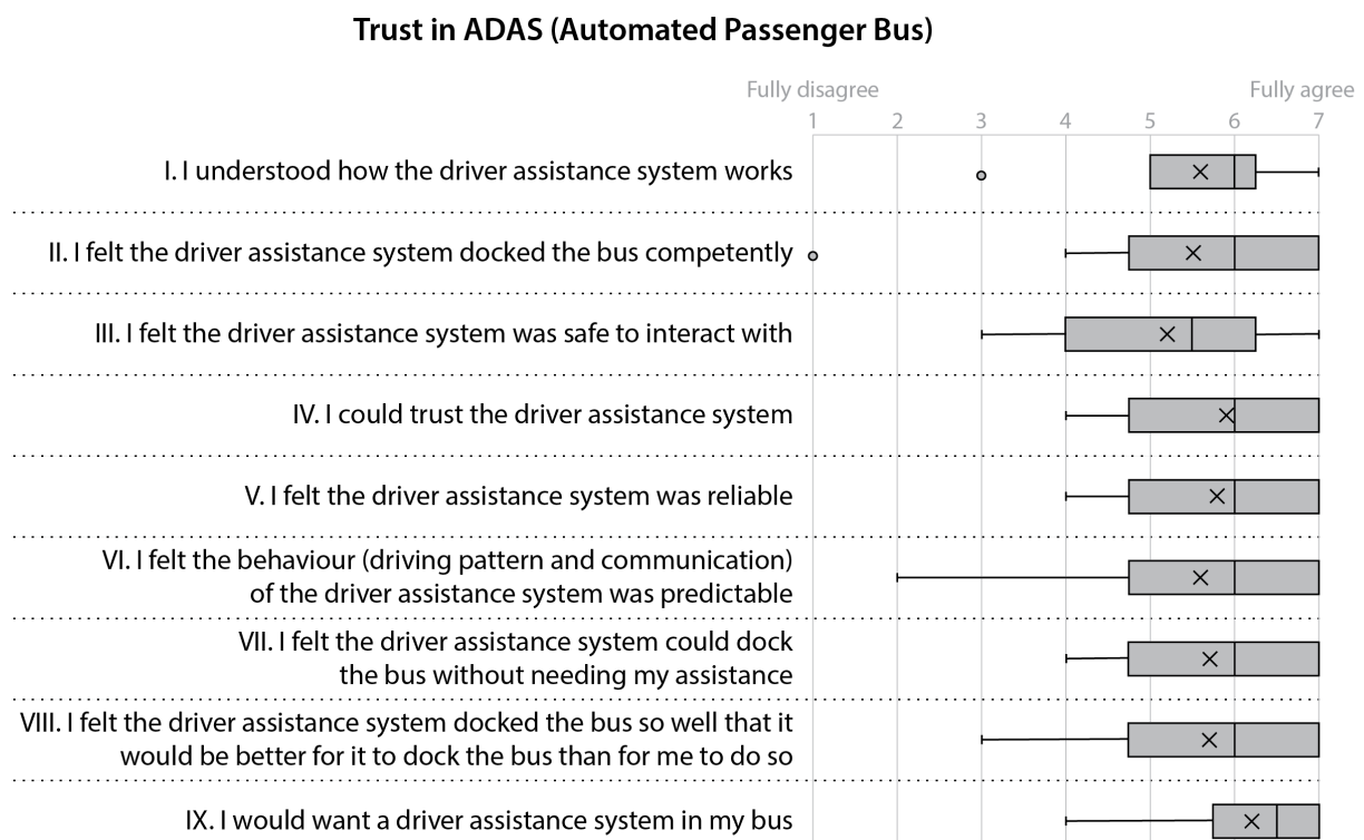
Figure 9 - Trust-questionnaire results
