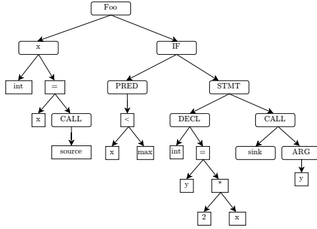
Figure 1.1: Abstract syntax tree (AST) for the code snippet in Listing 1.
