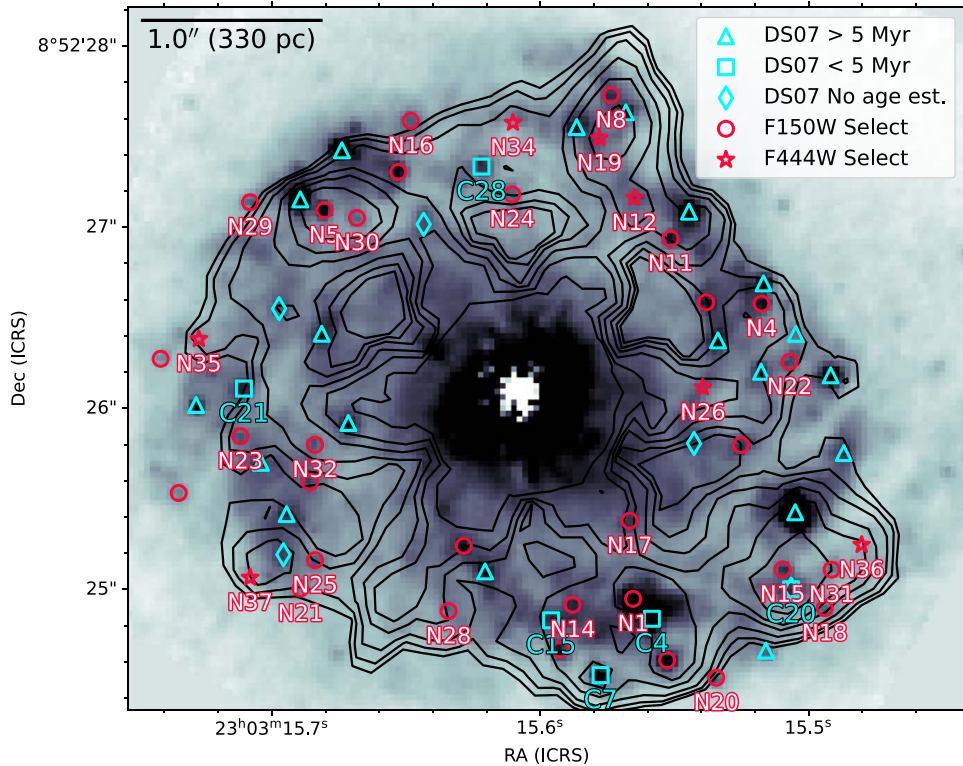
Figure 3. NIRCcam/F150W image where F150W-selected and NIRCcam/F444W-selected star-forming regions with red colors ( F200W/F150W > 1.1 or F444W/F200W > 2.5 ) are labeled. The markers are the same as Figure 2 and the contour levels show the MIRI/F560W emission. Groups of sources with red NIR colors are somewhat clustered in the north and southwest regions, which coincide with the peaks of MIR and radio emission. The markers sizes are not representative of the extraction sizes.
