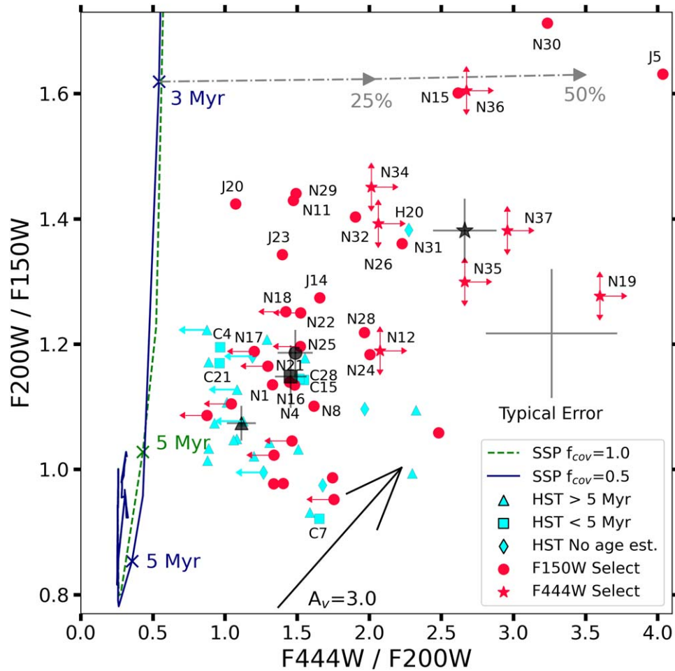
Figure 4. NIRCam F200W/F150W vs. F444W/F200W color-color plot of the starburst ring of NGC 7469. The markers follow that of Figure 3, where red sources, F200W/F150W > 1.1 or F444W/F200W > 2.5 , are labeled. Sources with fluxes below the 3\sigma detection threshold are treated as upper limits for the associated filter. The median colors of each source group are shown with the same markers, but in black. Two single-stellar population models (the green dashed line with f_{cov} , the fraction of ionizing photons, equal to 1.0 and the dark blue solid line with f_{cov} = 0.5 ) are also shown, where the crosses denote the locations where the stellar age is 3 and 5 Myr. The typical error and an attenuation vector representing A_V = 3.0 are included. The positions of the arrows indicate fractional contributions of 25% and 50% to the F444W flux. The majority of the JWST sources with red colors likely have young (3–5 Myr) stellar populations that are highly obscured and contain large amounts of hot dust.
