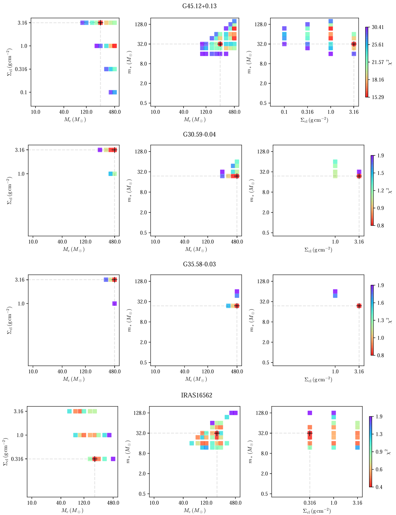
Figure A4. Diagrams of the \chi^2 distribution in the \Sigma_{\text{cl}}-M_c space (left column), m_*-M_c space (center column), and m_*-\Sigma_{\text{cl}} space (right column) for each source noted on top of each plot. The black cross is the best model.
