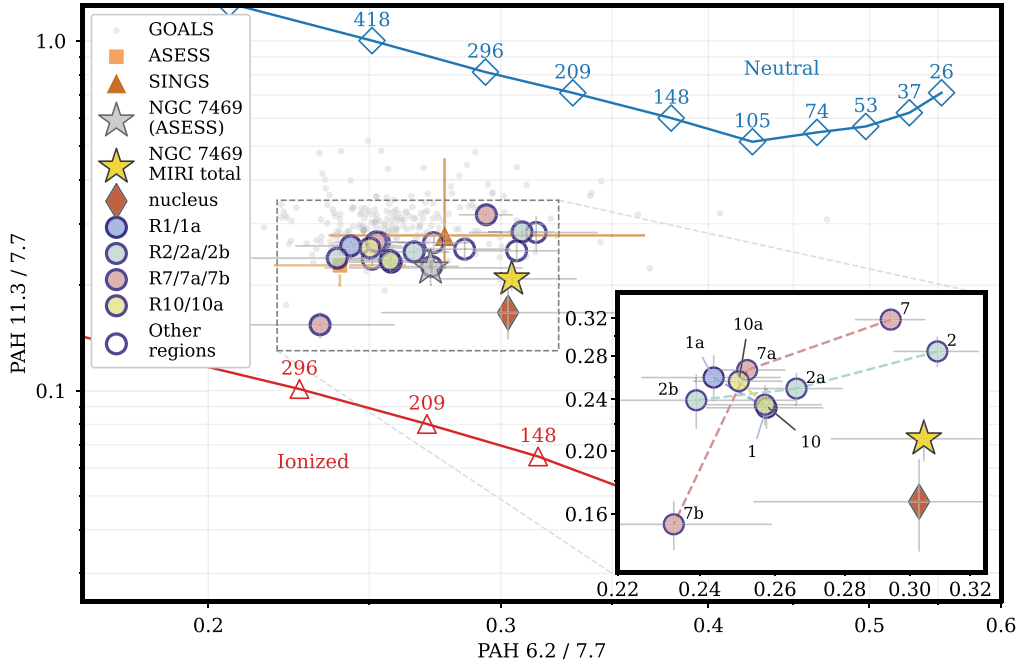
Figure 3. The interband ratios of the three main polycyclic aromatic hydrocarbon (PAH) bands at 6.2, 7.7, and 11.3 \mu\text{m} in the 17 regions extracted from the star-forming ring. The two tracks indicate the theoretical values for neutral and ionized PAHs with corresponding numbers of carbon atoms from Draine et al. (2021a). The star symbol indicates the PAH ratios derived from the total extraction of NGC 7469 in the MIRI MRS (Armus et al. 2022), while the red diamond is the ratio derived from the central nucleus. For comparison, the galaxies in GOALS (Stierwalt et al. 2014) are shown in gray points, along with points showing the 20%–80% range in star-forming galaxies from surveys of ACESS (Lai et al. 2020) and SINGS (Smith et al. 2007). The gray star indicates the measurement of the combined AKARI +Spitzer spectrum of NGC 7469 in ACESS. (inset) The zoom-in of the regions used for radial variation studies. Regions with a and b designations are those close to the nucleus as shown in Figure 1(b). Every region in the inset shows a trend of decreasing PAH 6.2/7.7 ratio when progressively moving toward the center, suggesting an increase of the grain size distribution.
