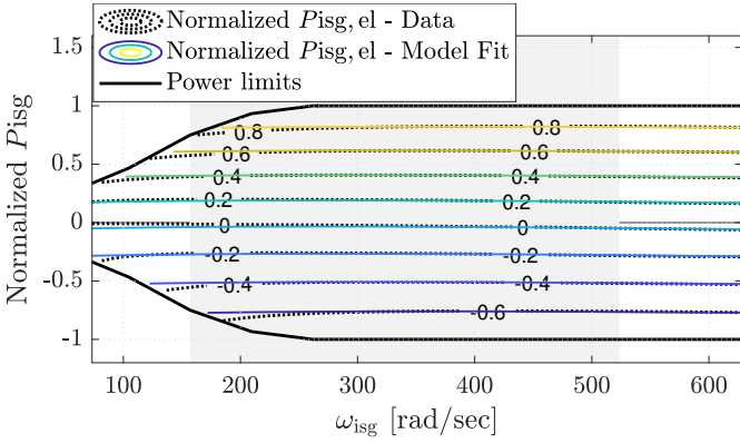
(b) Normalized values of the measured (dotted line) and the estimated (solid line) electrical power consumption of the ISG, P_{issg,el} , illustrated as contours.
