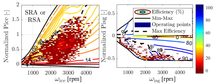
Fig. 10: Actuator operating point distribution of the proposed strategies with 3\lambda_b , i.e., 3 times the value of co-state used to obtain the results in Fig. 9. The hot-spot (colors in the range between red and orange) of the ICE operating points are now closer to the maximum efficiency line and are grouped at higher speeds (around 3000 rpm), compared to the values in Fig. 9. The ICE delivers entire or major part of the propulsive demand whereas the ISG is either in generation or regeneration mode.
