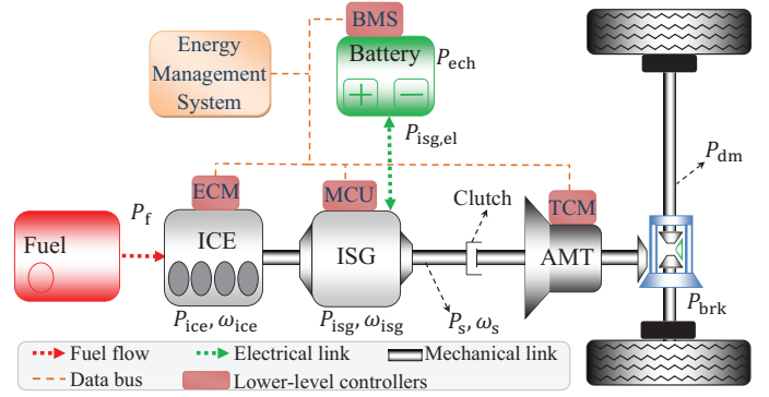
Fig. 1: The considered parallel HEV powertrain consists of an ICE and an ISG connected to the wheels via an 8-speed auto-transmission, where P_{brk} is the braking power demanded. The Energy Management System hosts the proposed supervisory co-optimization controller (SCC) which sends optimal references to each of the lower-level controllers.
