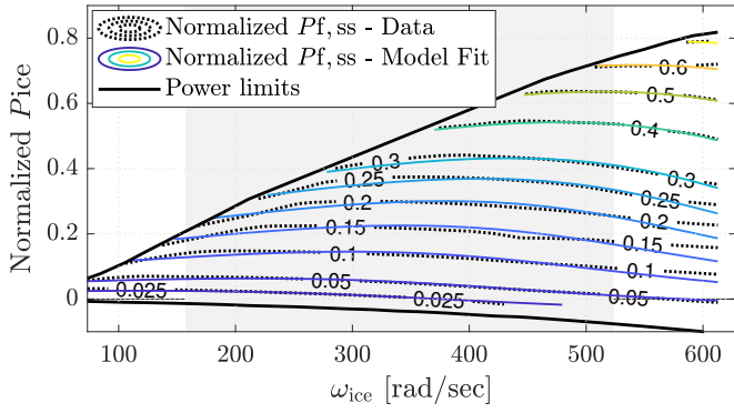
(a) Normalized values of the measured (dotted line) and the estimated (solid line) gasoline consumption of the ICE, P_{f,ss} , illustrated as contour lines.
