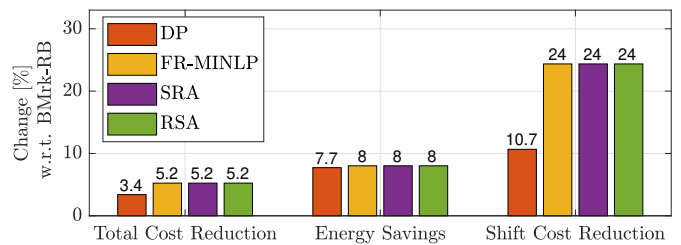
(a) This bar graph shows cost comparison over a single MPC update with a prediction horizon t_h = t_f - t_0 . The solutions of the proposed strategies, SRA and RSA, lie between the solutions of the FR-MINLP (lower bound of (39)) and the DP (upper bound of (39)) strategies, respectively.
