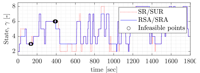
Fig. 11: Plot showing the infeasibility issue in known standard rounding (SR) and sum-up rounding (SUR) strategies [32], [33] against the proposed strategies, under WLTC Class-3b drive cycle. Blue solid line shows the gear trajectory for RSA and SRA strategies whereas the red dotted line shows the trajectory for the known rounding strategies being compared. Black circles around 140 sec and 390 sec show the instances where the usage of SR and SUR resulted in infeasible gear values in which the actuators were not able to deliver the demanded power. Notice that at these instances the proposed strategies have chosen a gear lower than the rounding strategies to ensure feasibility of the solution.
