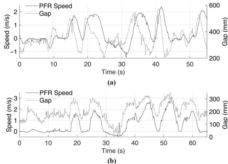
Figure 8 The following gaps and PFRs speeds of test records: (a) the linear model; (b) the OVM/FVDM
