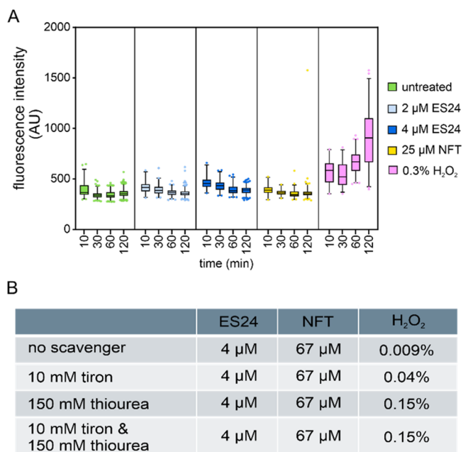
Figure 2. Oxidative stress assays. (A) Oxyburst Green assay for detecting ROS in B. subtilis 168CA. The fluorescent probe shows a marked increase in fluorescence when ROS are present. It should be noted that Oxyburst Green has been reported to be specific for the detection of superoxide, yet we have found that it reacts to different sources of ROS (see Figure S2). (B) Influence of ROS scavengers on antibiotic activity against B. subtilis 168CA. MICs were determined in the absence or presence of the superoxide scavenger tiron or the hydroxyl radical scavenger thiourea. If one of these ROS species contributes to the activity of the compound, the MIC should increase in the presence of the respective scavenger.
