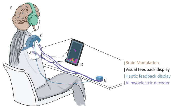
Figure 2 Schematic illustration of the setup used in a participant with amputation and nerve injury (eg, brachial plexus injury). Myoelectric signals are recorded through surface electrodes (A) and decoded by a myoelectric pattern recognition decoder (B). The acquired signals are processed by a custom software. A user-interface is displayed on a screen providing the participant with instructions and virtual environment related to the therapy. Tactile (C) and/or visual (D) feedback is perceived as a response to the movement. Concurrent to performing the training, the brain modulation is used by a transcranial direct current stimulation system (E).
