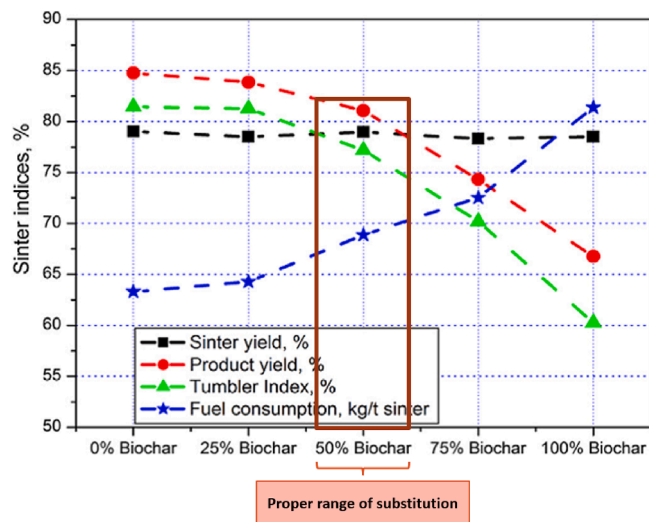
Fig. 4. Impacts of biochar addition on sinter indices [69].
