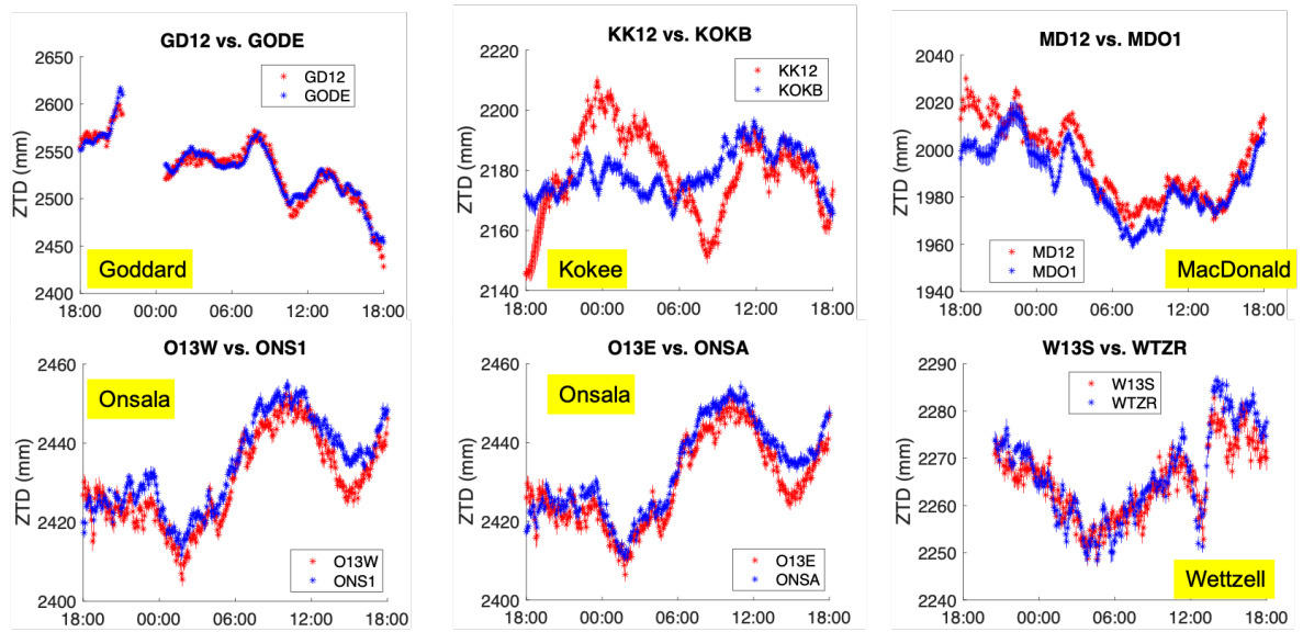
Fig. 5 Time series of ZTD with a 5-minute temporal resolution from VGOS (red) and GNSS (blue), respectively, for the six sites participating in VR2101 that had both techniques operating.
