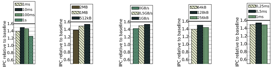
Fig. 13: Sensitivity analysis.
