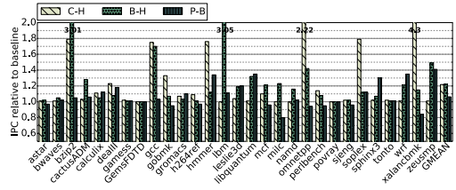
(b) Performance improvement from increasing cache allocation to 2MB (C-H), and increasing bandwidth allocation to 16GB/s (B-H) in comparison to the baseline allocation, with prefetching disabled. Performance improvement from enabling prefetching for the baseline allocation (P-B).
