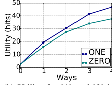
(b) Utility for '1' and '0' in the square-and-multiply algorithm.
