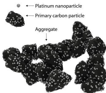
Figure 3.2: Illustration of carbon supported platinum catalyst particles. Pt nanoparticles are dispersed on the surface of primary carbon particles, which forms aggregates together that creates a porous structure.
