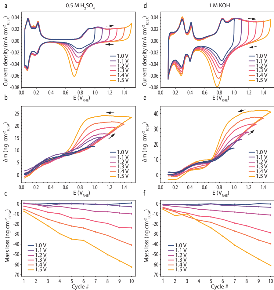
Figure 5.1: CVs, corresponding mass responses and mass loss per cycle of Pt thin films cycled to different upper potential limits in 0.5 \text{ M H}_2\text{SO}_4 (a, b and c) or 1 \text{ M KOH} (d, e and f) at 50 \text{ mV s}^{-1} and under inert atmosphere.
