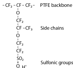
Figure 3.4: Chemical structure of Nafion.
