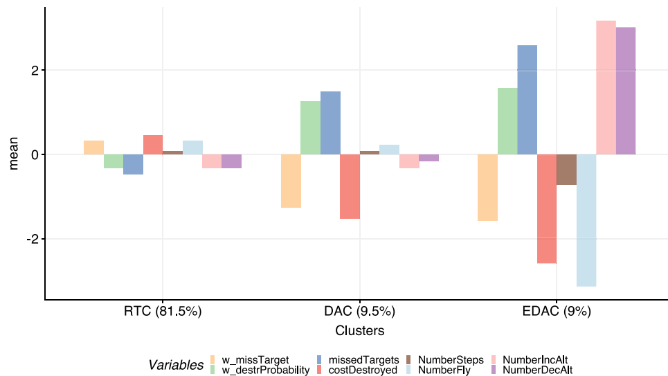
Fig. 13. Bar plot of the cluster means for DARTSim.
