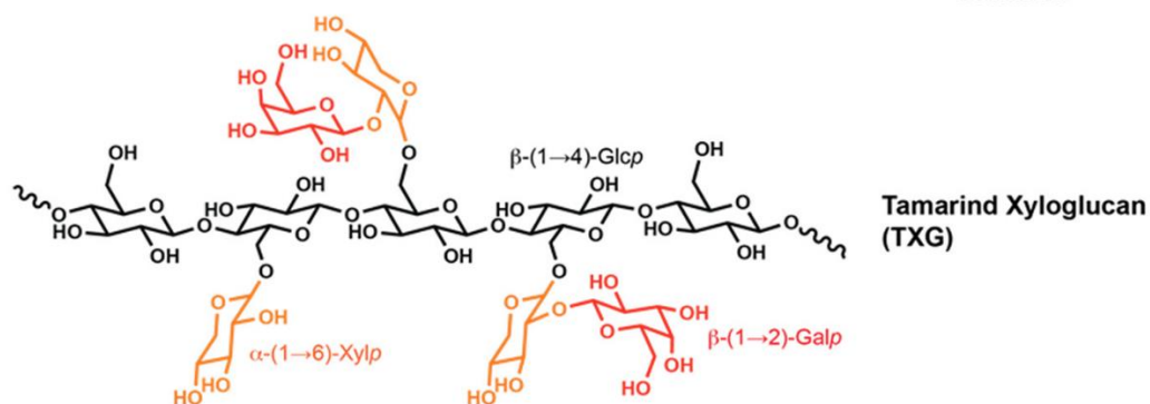
Figure 7. Chemical structure of xyloglucan from tamarind seeds. The \beta -1,4-glucopyranosyl (Glc p ) backbone is shown in black, whereas the \alpha -1,6-linked xylopyranosyl (Xyl p ) decorations are shown in orange and the \beta -1,2-galactopyranose (Gal p ) residues in red. The figure was retrieved from Paper II under the CC BY 4.0 license (and slightly modified).
