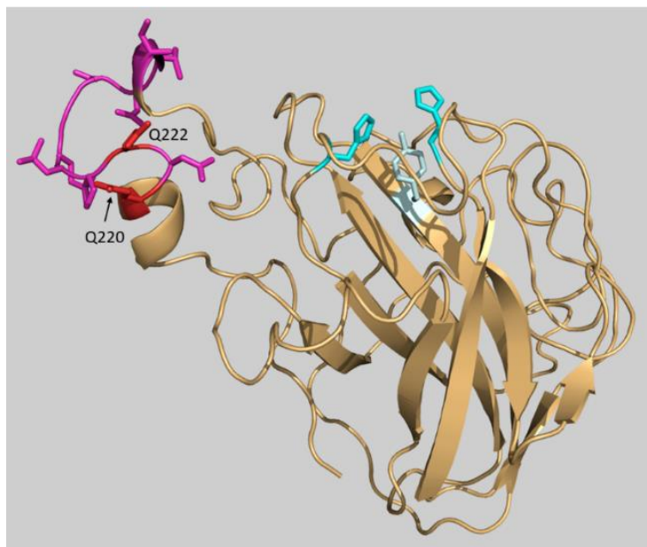
Figure 18. A PyMol model of Tt LPMO9U illustrating the extra loop in the 214–224 region (in magenta). The polar glutamine residues are colored in red and the histidine brace in cyan, whereas the Tyr in the proximal axial coordination position is colored in light blue. Modelling and figure courtesy to Dr Olav A. Hegnar.
