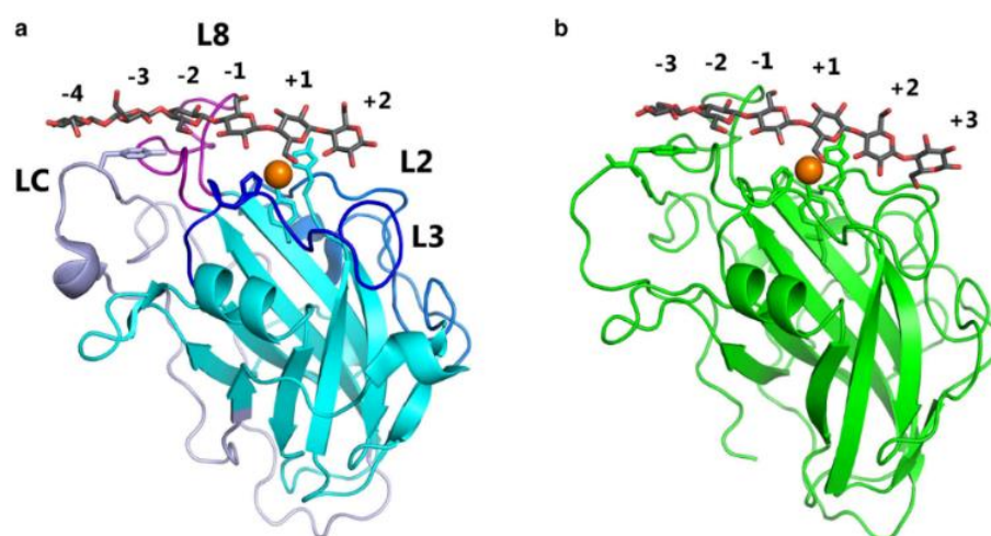
Figure 17. X-ray crystal structures of Lentinus similis LsLPMO9A (a) and Collariella virescens CvLPMO9A (b) forming a complex with cellobiohexaose (grey carbons). The numbers indicate substrate-binding subsites. The Cu atom is shown as an orange sphere. For LsLPMO9A, substrate-binding loop C-terminal (LC), L2, L3, and L8 regions are marked. The figure was retrieved from (190) under the CC BY 4.0 license.
