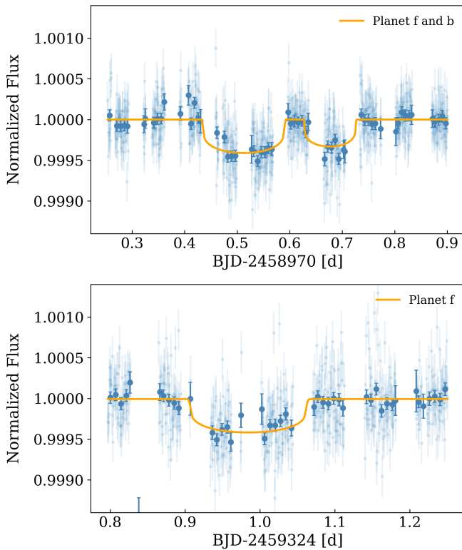
Fig. 3. CHEOPS light curve of HD 108236 during a transit of planet f ( \sim 2458970.5 BJD) and b ( \sim 2458970.7 BJD) (top panel), as well as during a dedicated observation of a planet f transit (bottom panel). Detrended photometric points and its 10 min bins are represented by light and dark blue dots, respectively. The best model for each planet is represented by the yellow curve.
