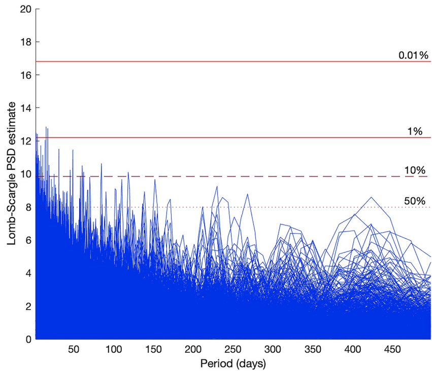
Figure B3. Lomb-Scargle PSD estimates of 1,000 signals comprised purely of Gaussian noise, rescaled, and resampled to match the magnitude of SO 2 emission rates reported and the days for which an SO 2 emission rate is available at Mayon volcano. FAPs are calculated with threshold values indicated for FAPs of 50% (8.0), 10% (9.9), 1% (12.2), and 0.01% (16.8).
