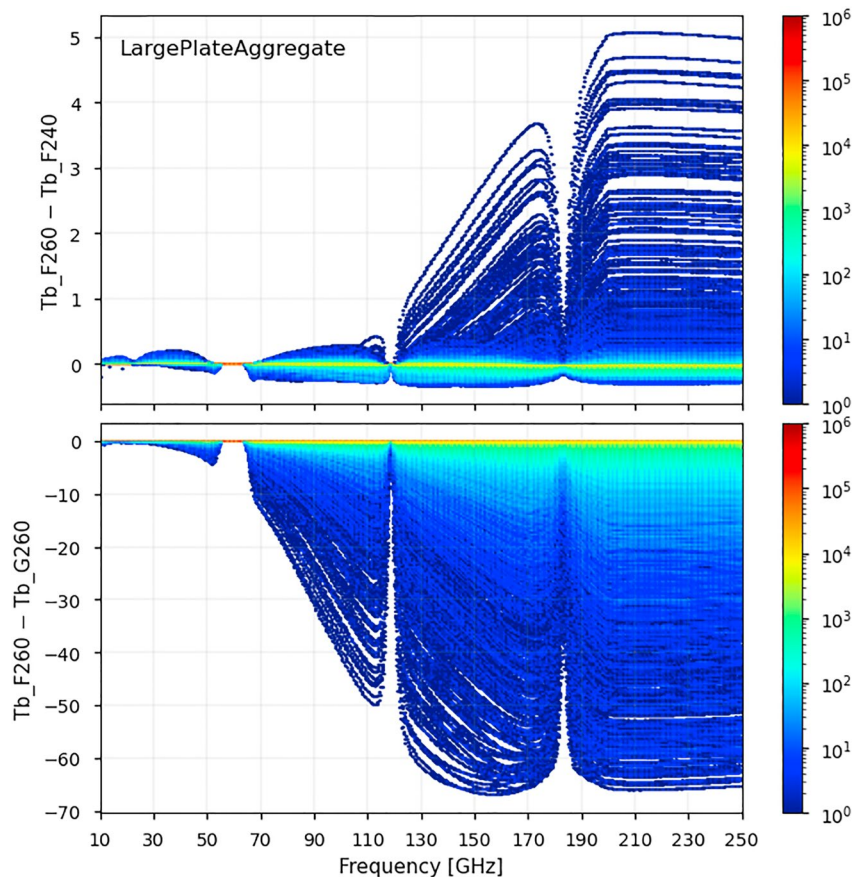
Figure 7. Difference in simulated brightness temperatures due to the choice of reference temperature or PSD used to generate the cloud lookup tables. The results are for all-sky simulations with LargePlateAggregate being used to prescribe the snow water content. Tb_F260 and Tb_F240 show the brightness temperatures simulated using lookup tables generated using Field et al. (2007) PSD and a reference temperature of 260 and 240 K, respectively, and Tb_G260 shows the brightness temperatures simulated using a reference temperature of 260 K and Zhou et al. (2022) PSD. The colorbars show number of occurrences as a function of channels' frequency.
