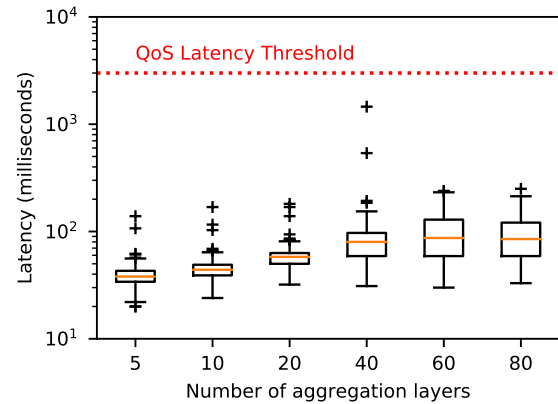
Figure 6: Boxplots of the latency values observed when clustering a different number of layers using the query in Alg. 1.
